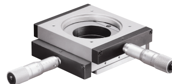
Slide Guidances with transmitted Light Opening
